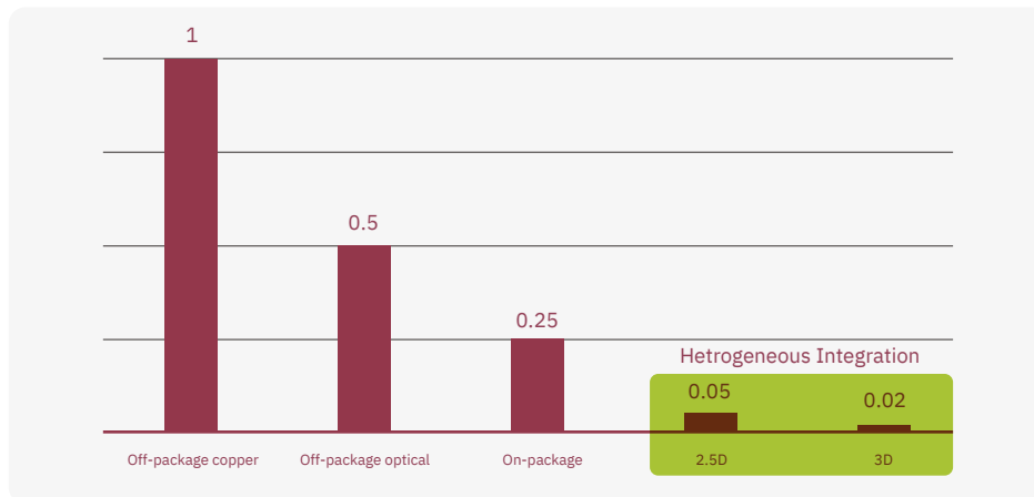
Relative Joules/Bit
