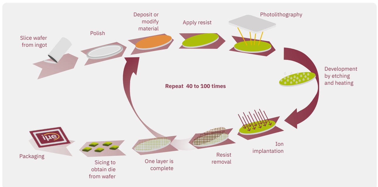
Semiconductor production process. 9
